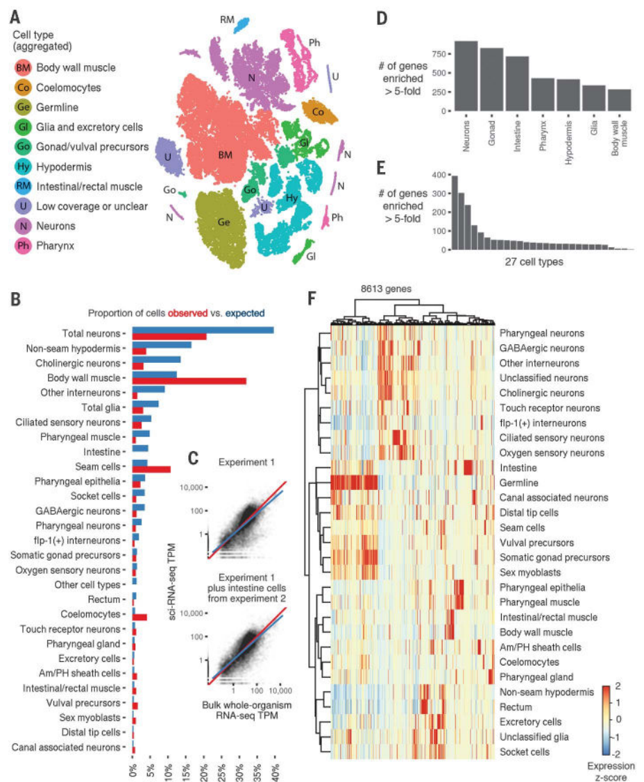
Fig. 3. A single sci-RNA-seq experiment highlights the single-cell transcriptomes of the C. elegans larva. (A) t-SNE visualization of the high-level cell types identified. (B) Bar graph showing the percentage of somatic cells profiled in the first sci-RNA-seq C. elegans experiment that could be identified as belonging to each cell type (red), compared with the percentage of cells from that type expected in an L2 C. elegans individual (blue). (C) Scatter plots showing the log-scaled transcripts per million (TPM) values of genes in the aggregation of all sci-RNA-seq reads (x axis) or in bulk RNA-seq (y axis; geometric mean of three experiments). Red line, y = x ; blue line, linear regression. The top plot includes only the first sci-RNA-seq experiment. The bottom plot also includes intestine cells from the second sci-RNA-seq experiment. (D) Number of genes that are at least five times as highly expressed in a specific tissue as in the second-highest-expressing tissue, excluding genes for which the differential expression between the first- and second-highest expressing tissues is not significant ( q > 0.05 ). (E) Same as (D), except comparing cell types instead of tissues. (F) Heat map showing the relative expression of genes in consensus transcriptomes for each cell type, estimated by sci-RNA-seq. Genes are included if they have a size factor-normalized mean expression of >0.05 in at least one cell type (8613 genes in total). The raw expression data (UMI count matrix) is log-transformed, column-centered, and scaled (using the R function scale), and the resulting values are clamped to the interval (-2, 2) . GABA, \gamma -aminobutyric acid.
